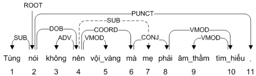
Figure 5. The final output dependency tree.
