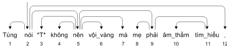
Figure 2. An unlabeled dependency tree converted from the tree in figure 1 in using the head rules for Vietnamese.
