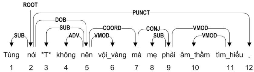
Figure 4. A coordination example.
