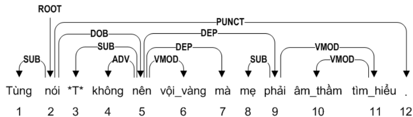
Figure 3. A labeled dependency tree transformed from the tree in figure 1 in utilizing the head rules and the algorithm 1.
